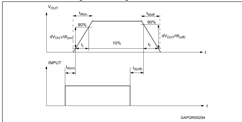
Figure 5. Switching characteristics
