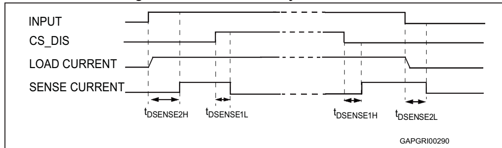
Figure 5. Switching characteristics
